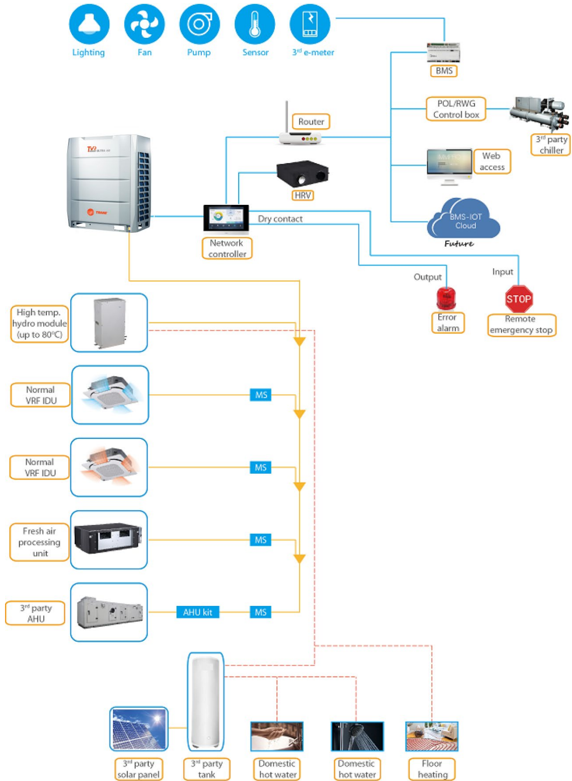
Figure 3.1: Hydraulic box connection method
