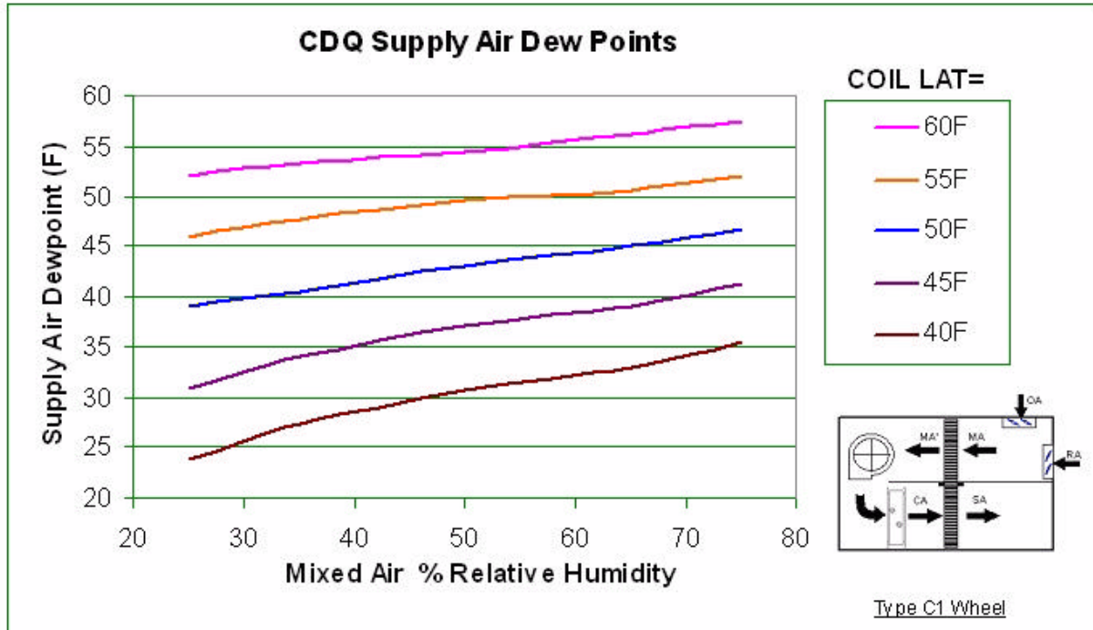
Figure 10. Typical achievable dewpoints
