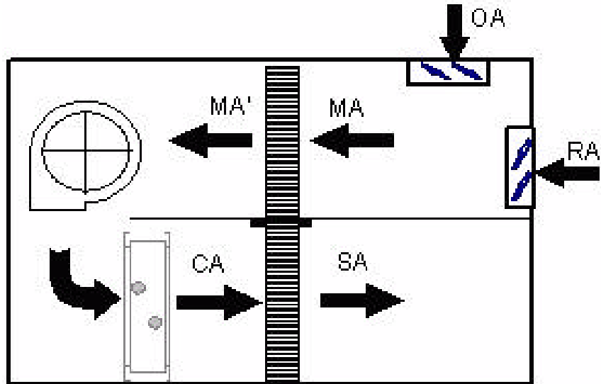
Figure 5. Basic CDQ™ air handler
