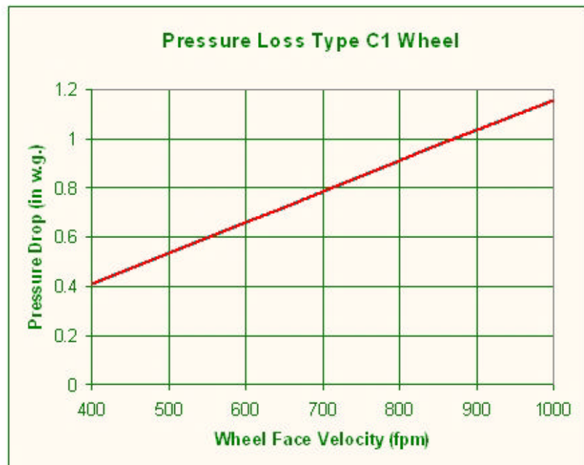
Figure 15. Type C1 wheel pressure drop
