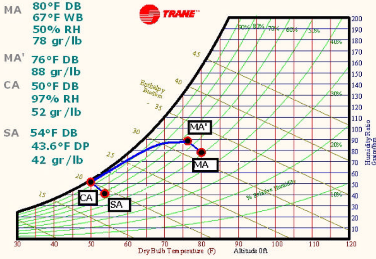
Figure 8. Sample performance and psychrometric plot
