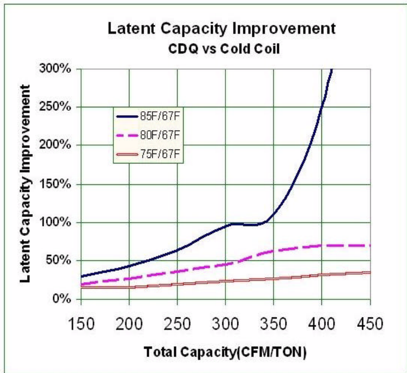
Figure 13. Latent capacity improvement
