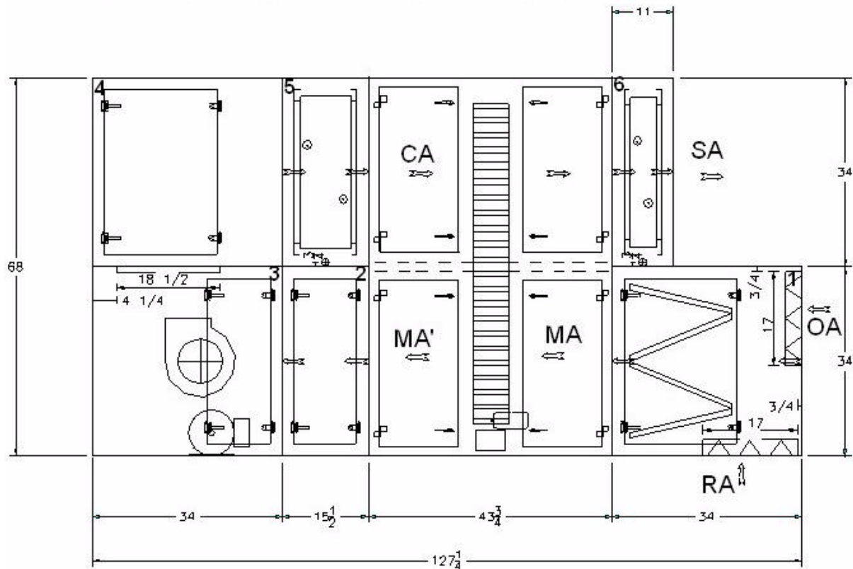
Elevation View Measurements in inches
