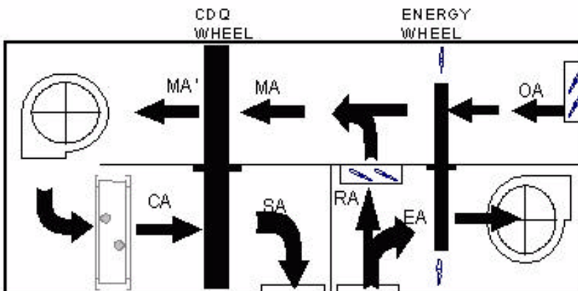
Figure 20. An example configuration for mixed air CDQ AHU with energy wheel
