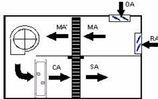
Figure 19. Supply fan locations
