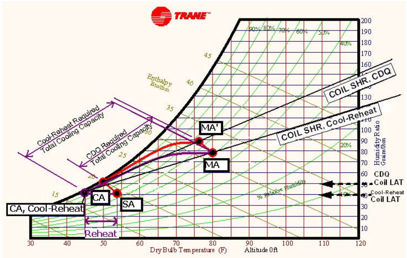
Figure 9. Psychrometric plot: A CDQ system vs. a cool-reheat system
