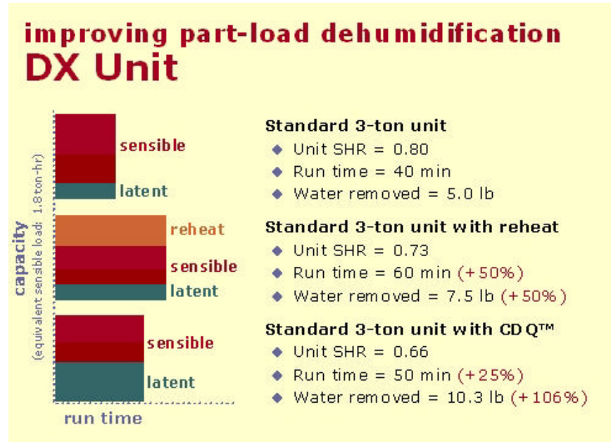
Figure 14. Example: Part load, 400 cfm/ton 80°F/67°F EA
