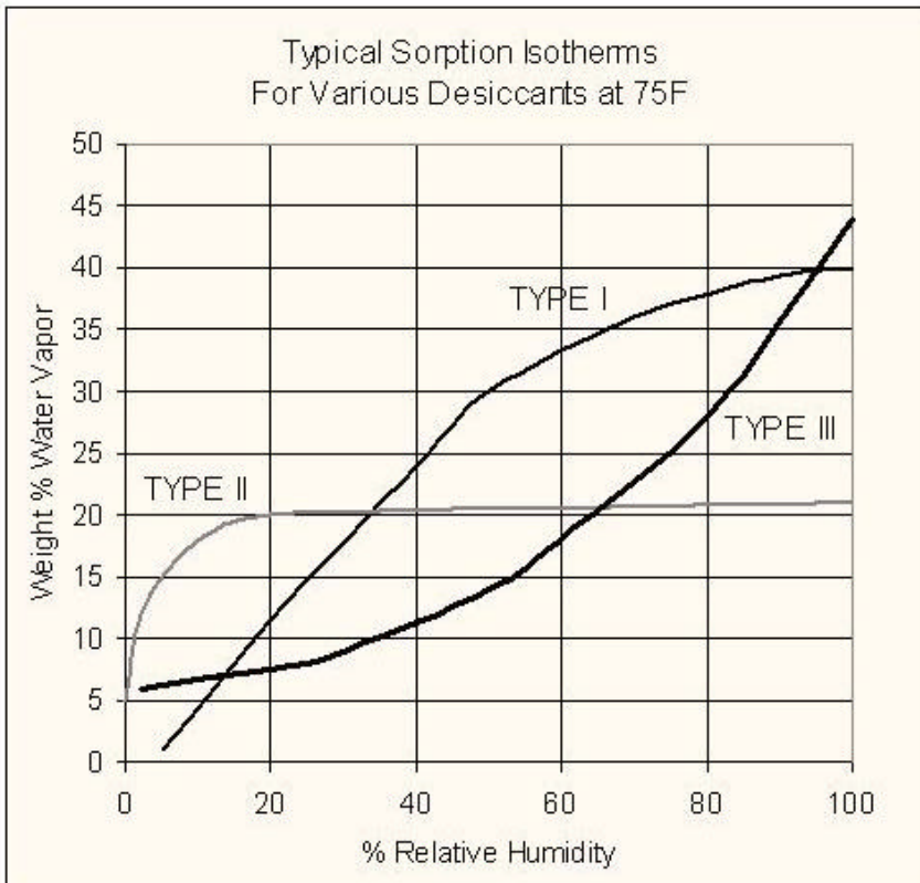
Figure 2. Example of desiccant isotherms
