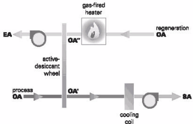
Figure 4. Active desiccant wheel
