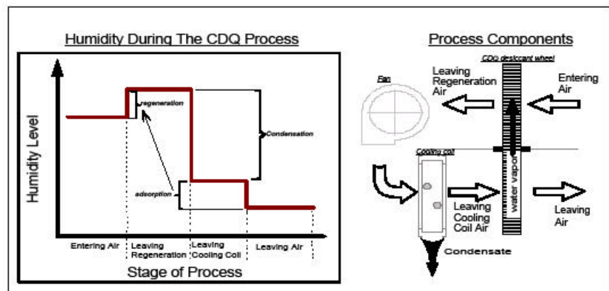
Figure 1. CDQ dehumidification processes
