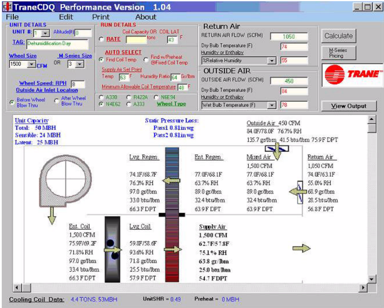
Figure 22. CDQ Performance Program example for dehumidification design conditions
