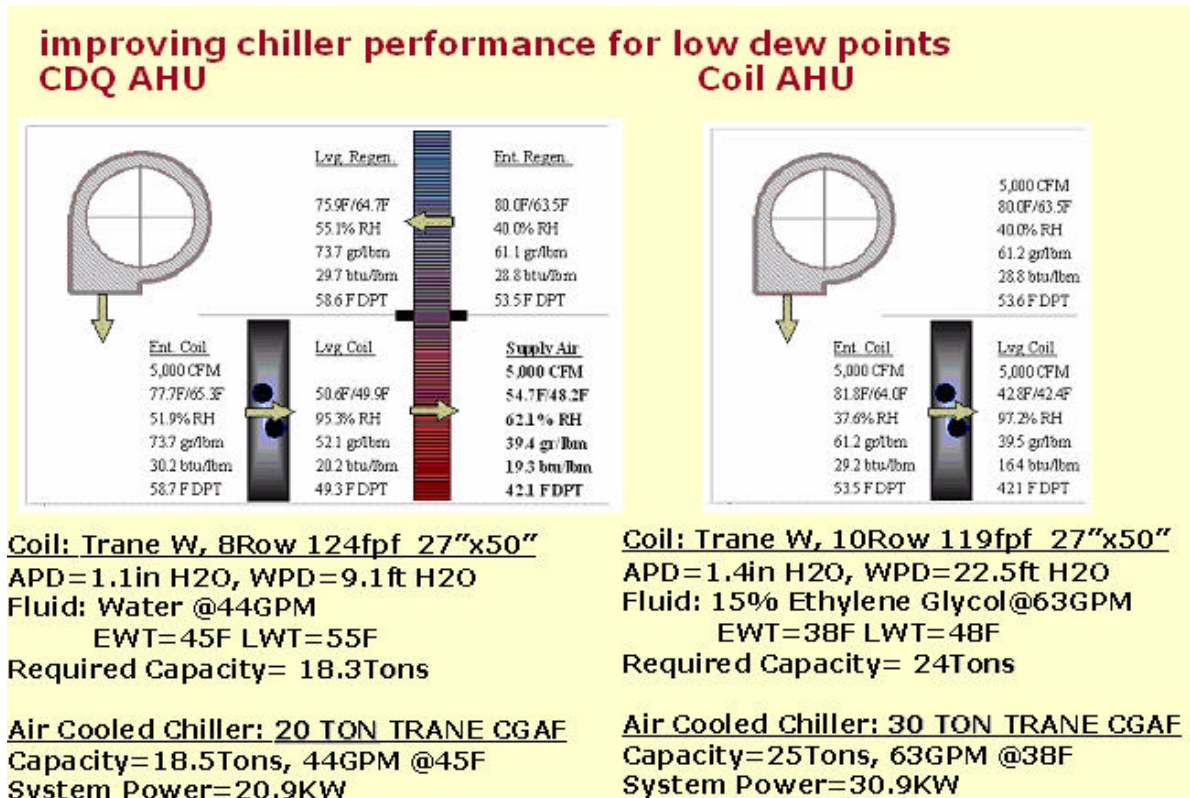
Figure 11. Improvement in cooling coil efficiency
