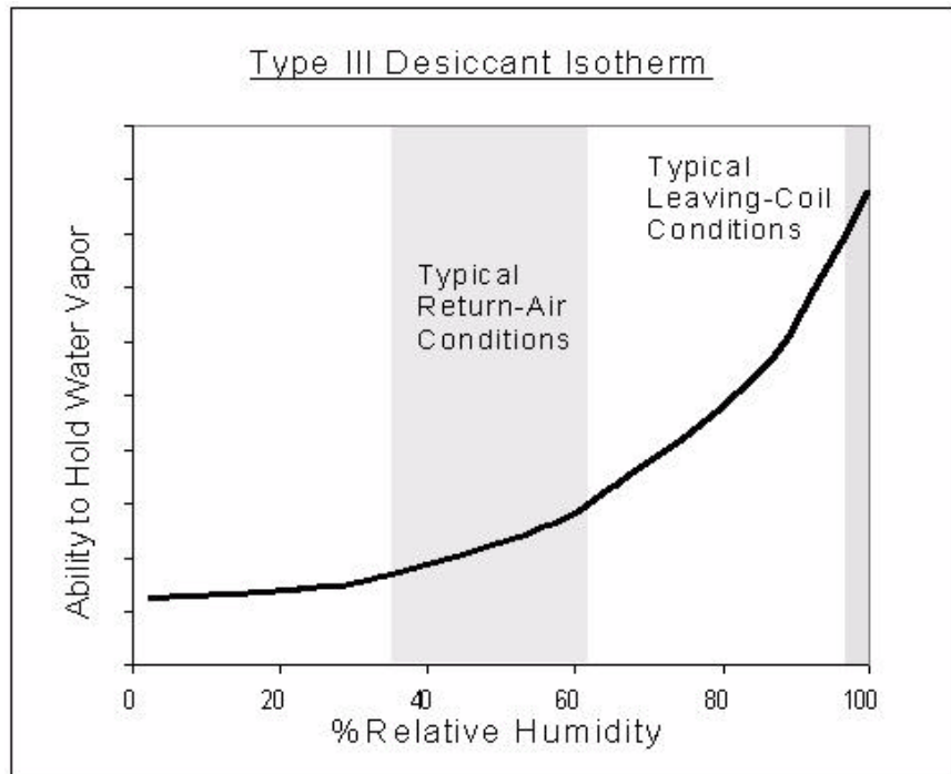
Figure 6. Type III isotherm and CDQ application
