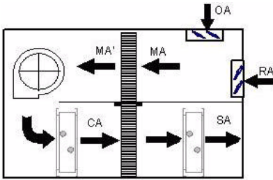
Figure 16. Sample air handler configuration
