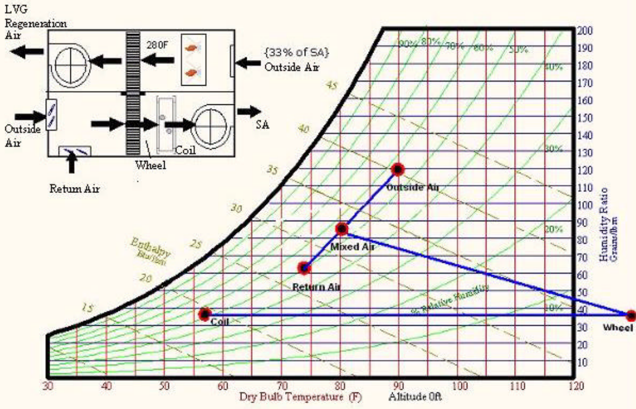
Figure 21. Example: Active desiccant system (eff = 1,950 Btu/lbm of water) 5,000 cfm, 80°F, 55% mixed air, 40°F supply-air dew point
