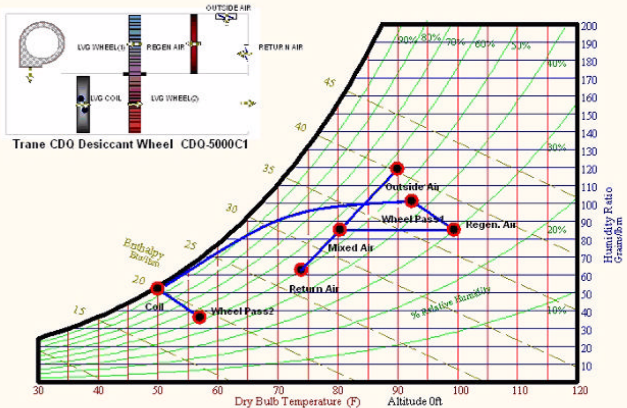
Figure 17. Example: Use of preheat, 5,000 cfm, 80°F, 55% mixed air, 40°F dew point
