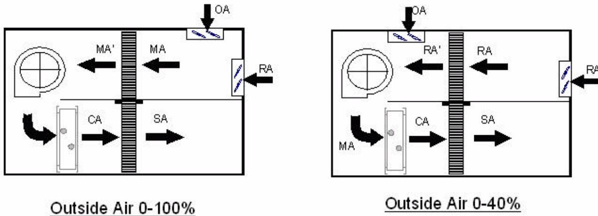
Figure 18. Acceptable outside air inlet locations
