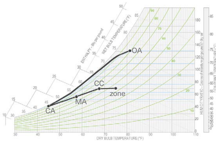
DOAS: 45°F supply air: Part load 0.667 SHR
