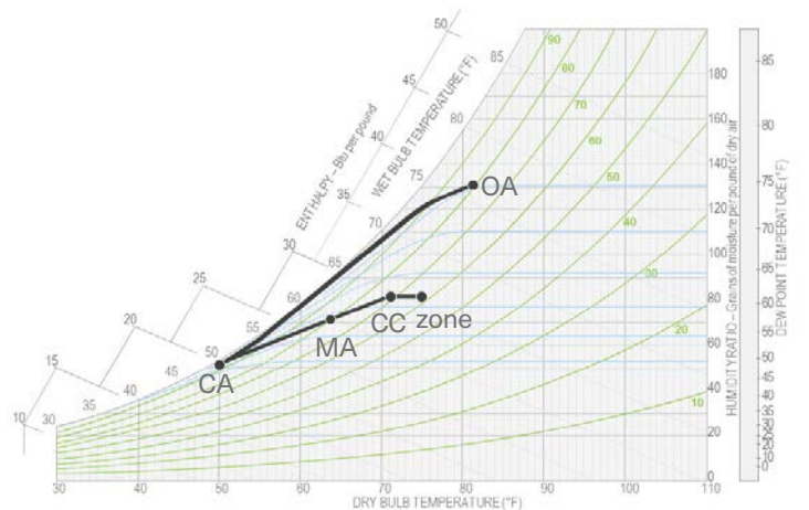
DOAS: 50°F supply air: Part load 0.611 SHR
