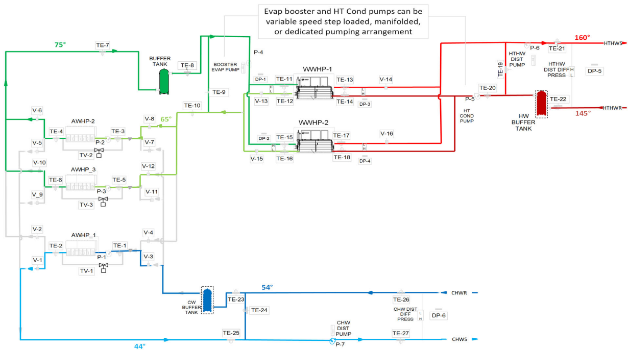
Figure 21. Cascade configuration
