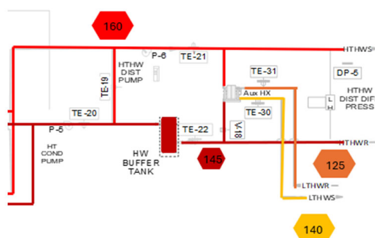
Figure 36. Dual temperature configuration with auxiliary heat exchanger
