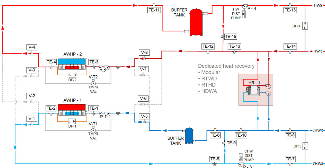
Figure 30. Dedicated heat recovery unit option
